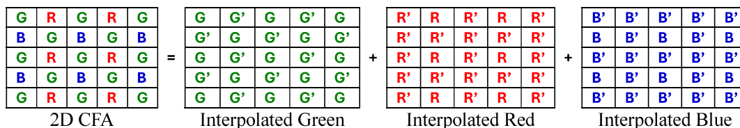
Figure 3 : Demosaicking/ Interpolation Process
